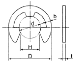
FIGURE B3 RETAINING RING (E-RING)
