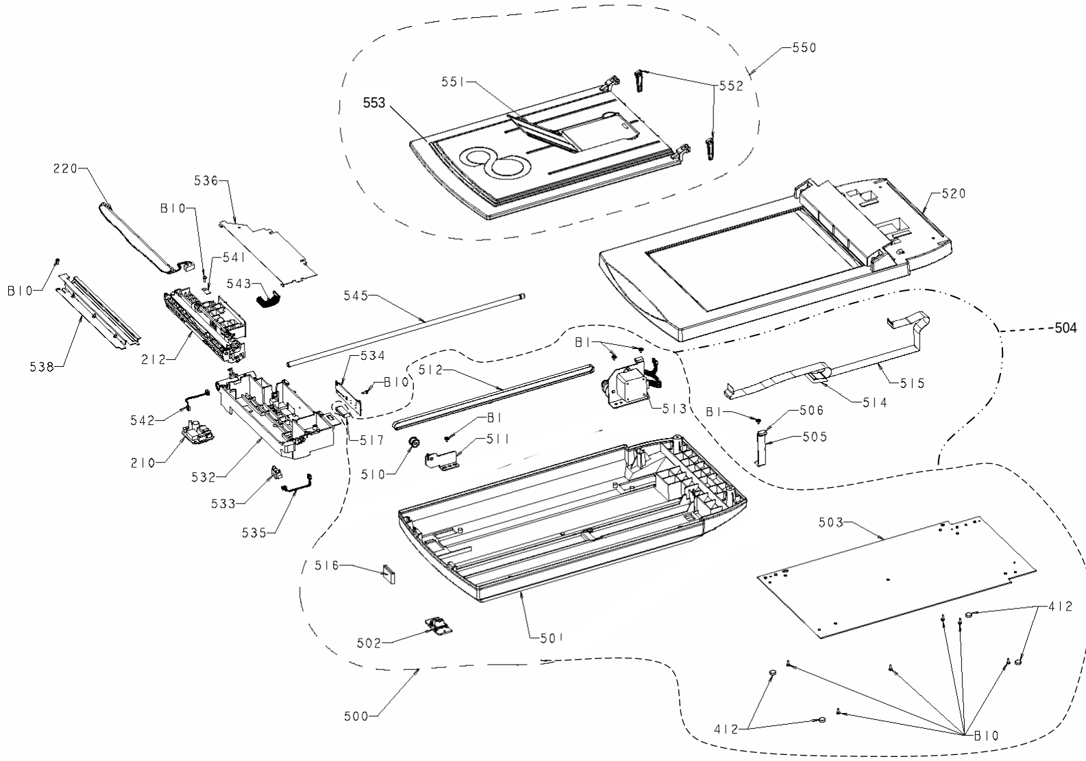
FIGURE 5. FLATBED
