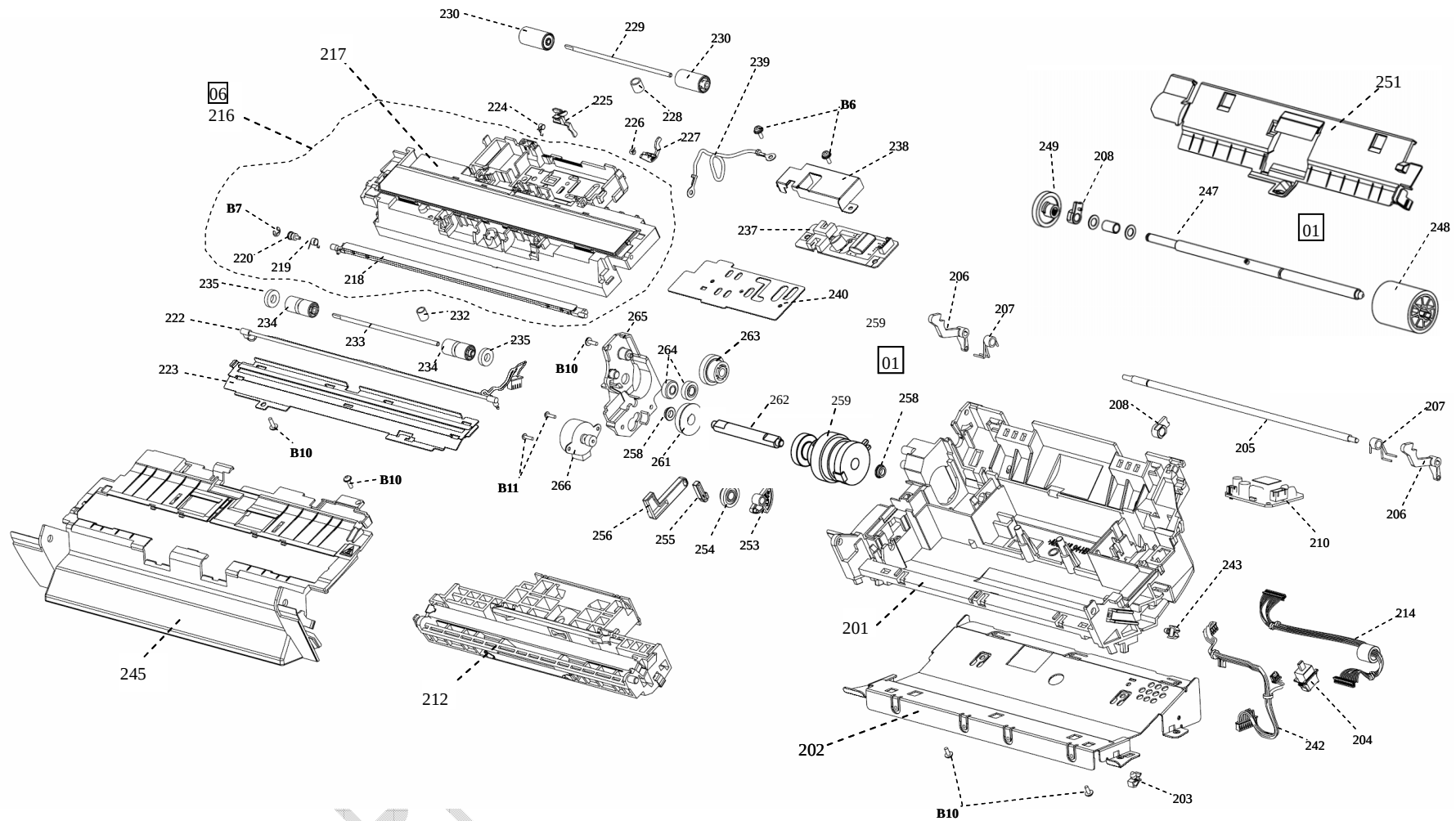
FIGURE 2. BASE UNIT
