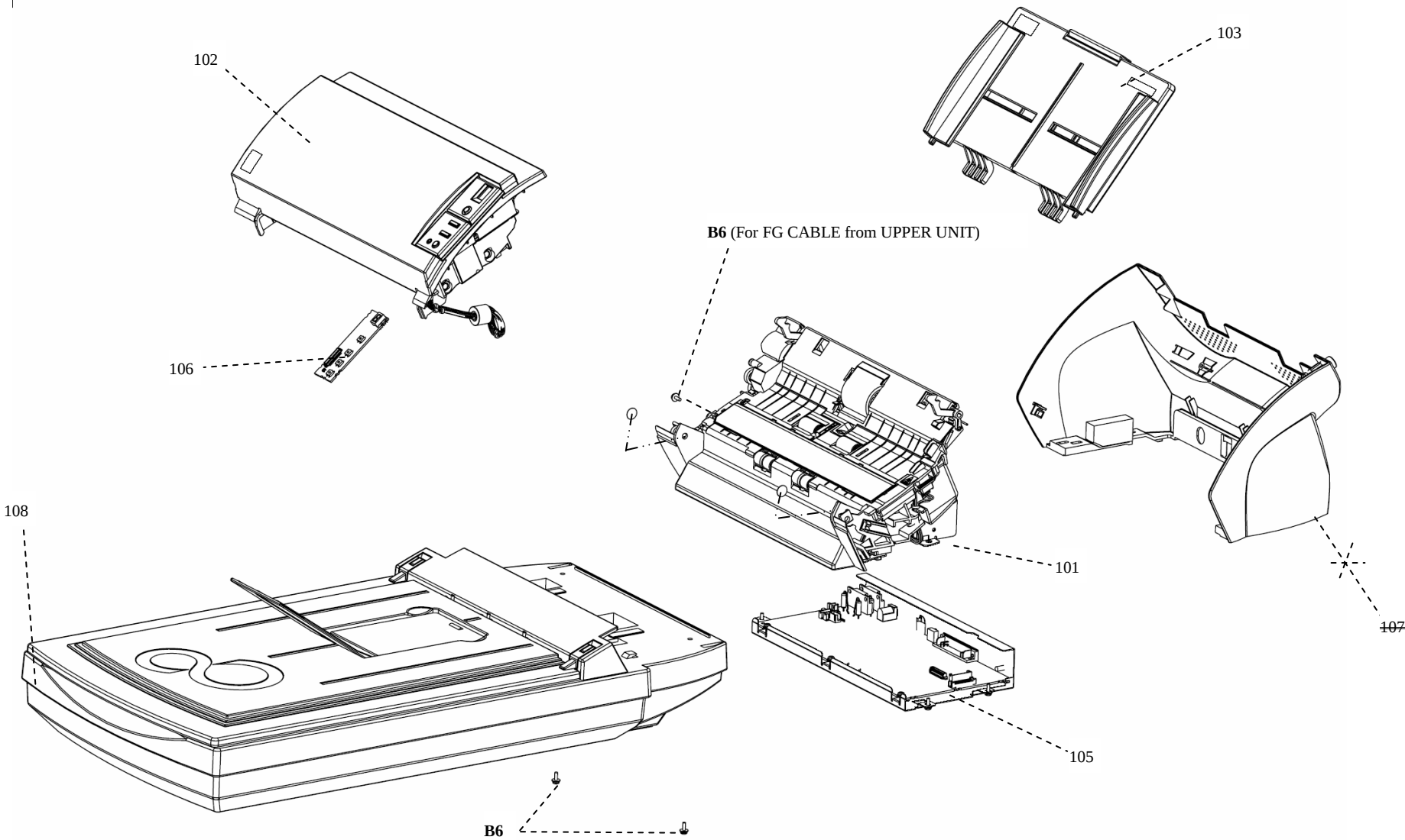
FIGURE 1. FINAL ASSEMBLY
